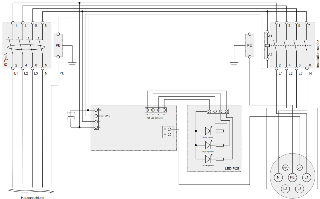
Abb. 4: Schaltplan LRT Home Essential Plus
